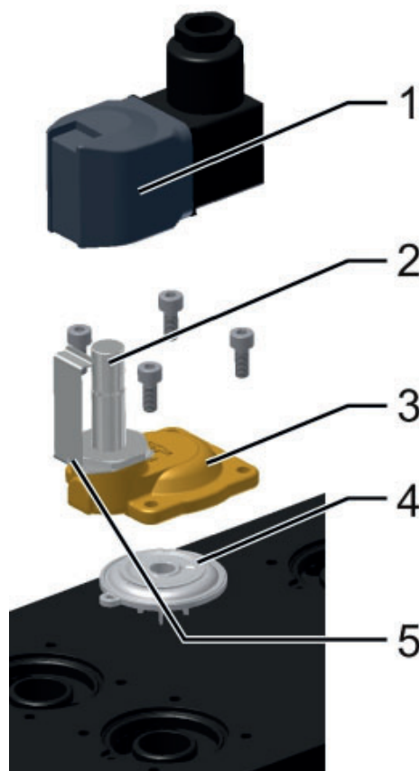
Solenoid valve
